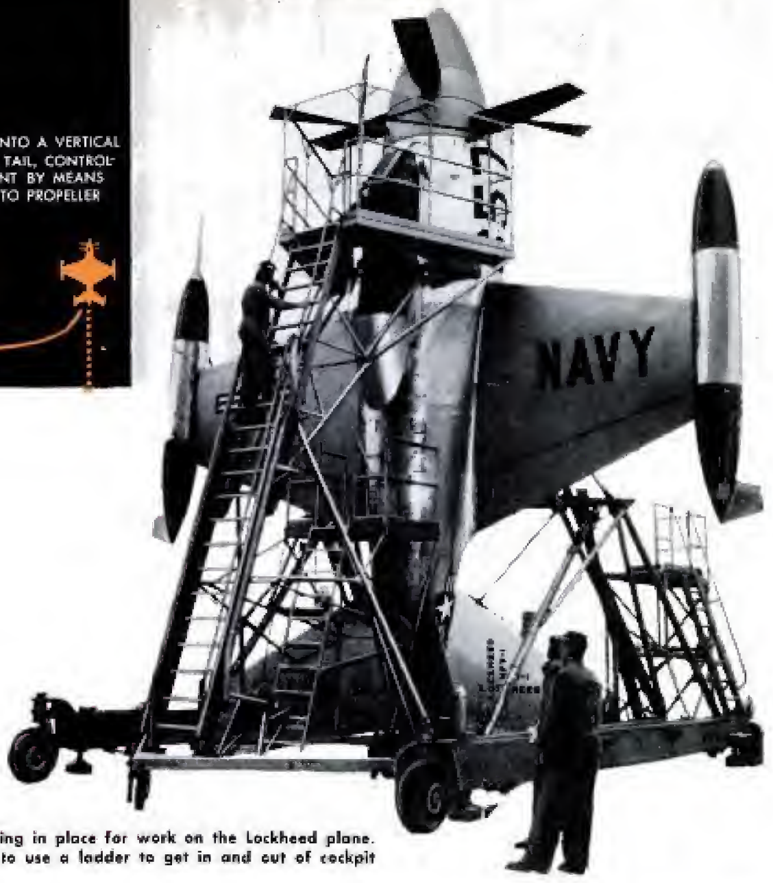
High, old-style landing gear will be used on the XFV-1 during its first test flights and then discarded
